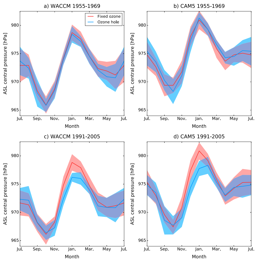
Figure 3. Seasonal cycle of ASL central pressure taken over 15 year periods: (a and b) the early period (1955–1969) before the effects of ozone depletion and (c and d) the late period (1991–2005) with the effects of ozone. Fixed ozone (red) and realistic ozone (blue) runs from WACCM4 (Figures 3a and 3c) and CAM5 (Figures 3b and 3d) are compared. The lines indicate the ensemble average and the shading represents the \pm 1\sigma of the yearly variability across the ensemble over the 15 year period.
