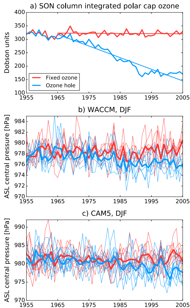
Figure 2. (a) Column-integrated polar ( 60\text{--}90^\circ\text{S} ) ozone in the Southern Hemisphere, averaged over September–November, used for the CAM5 runs with fixed ozone (red) and historic ozone levels (blue). The trendlines show trends over the period 1965–2005. Ozone levels for the individual WACCM members are shown in the supporting information Figure S1. (b) The ASL central pressure during DJF for six fixed ozone runs and six ozone hole runs in WACCM4 with the bold lines indicating the ensemble averages. (c) The ASL central pressure during DJF for eight fixed ozone runs and eight ozone hole runs in CAM5 with the bold lines indicating the ensemble averages.
