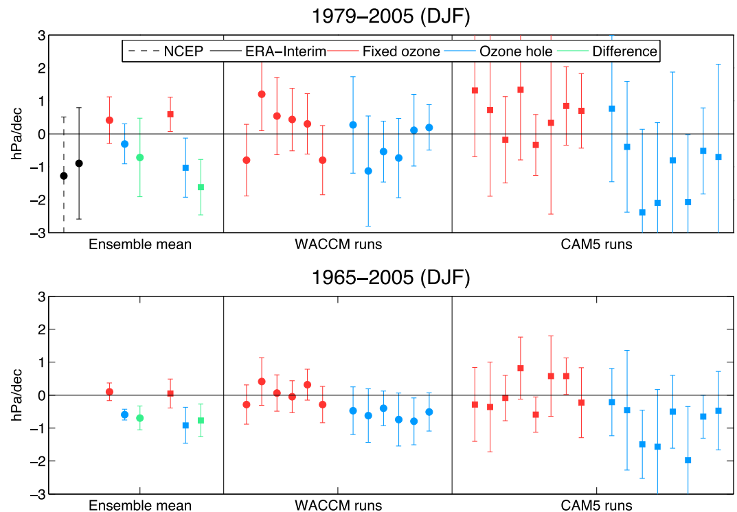
Figure 4. Trends in ASL central pressure in DJF during years (top) 1979–2005 and (bottom) 1965–2005. The ensemble average for both WACCM4 (circles) and CAM5 (squares) runs, as well as the individual members, are displayed with error bars indicating 95% significance. NCEP-DOE II and ERA-Interim are plotted for the shorter time period. Red indicates runs with fixed ozone levels, blue indicates runs with realistic ozone, and green shows the difference between them.
