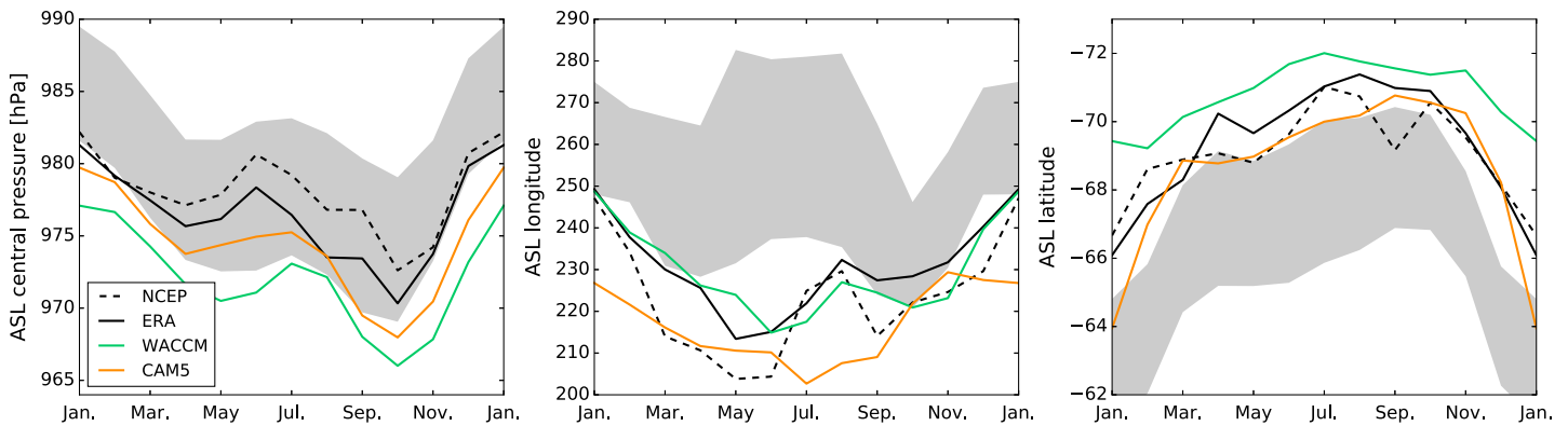
Figure 1. Seasonal cycle (average over 1979–2005) of three key metrics that define the Amundsen Sea Low: (left) central pressure, (center) longitude, and (right) latitude. An ensemble average of six WACCM4 (green) and eight CAM5 (orange) historical integrations are compared with NCEP-DOE II (dashed black) and ERA-Interim (solid black). The grey shading indicates the \pm 1\sigma envelope for 26 CMIP5 models.
